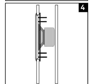
Speaker Installation As Viewed from Above
